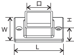
Oblong Base Plate
